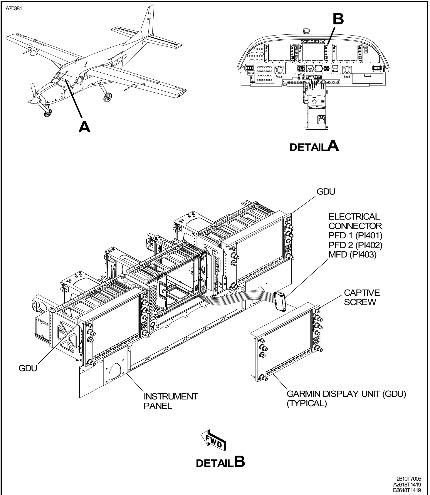
Figure 401 : Sheet 1 : Garmin Display Unit Installation
